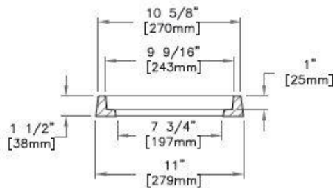
SECTION VIEW
